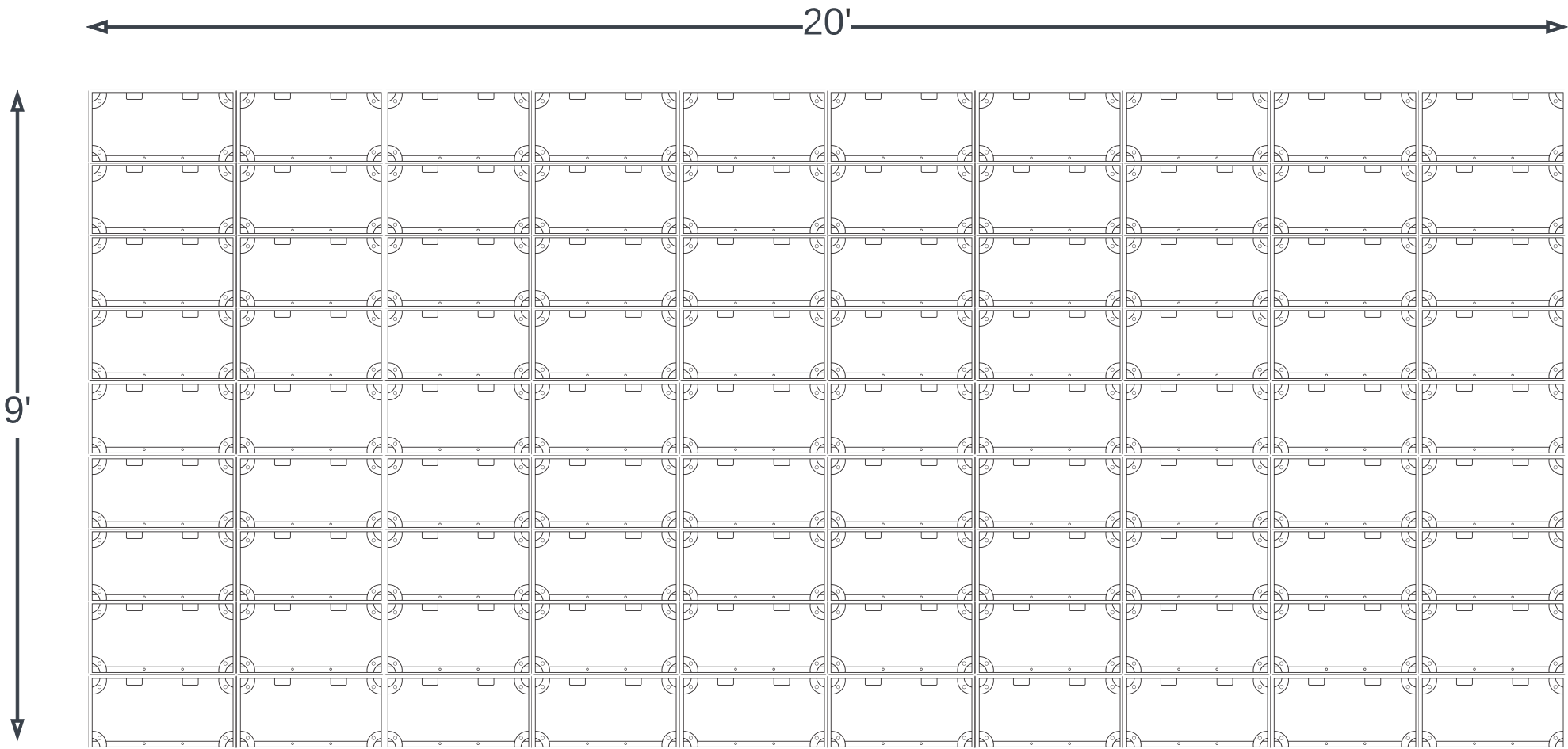
PRIMARY DISPLAY REARVIEW
